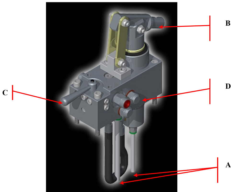
Fig.3.1: Main components of the hand pump
