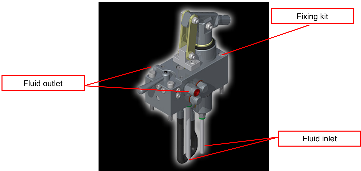
Fig.5.1: Hand pump - installation on tank
