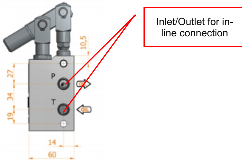
Fig.5.1: Hand pump – in-line installation
